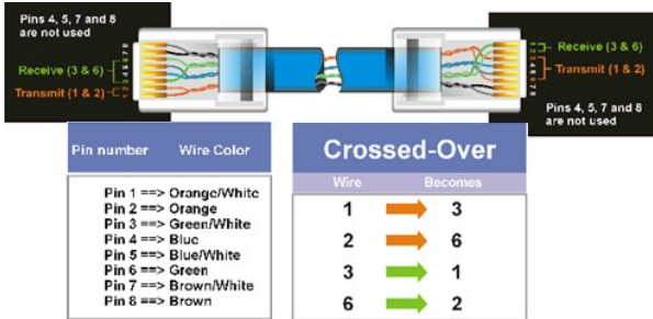
Pinout of crossover-cable
